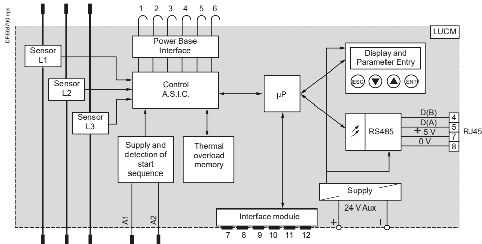
Basic scheme
